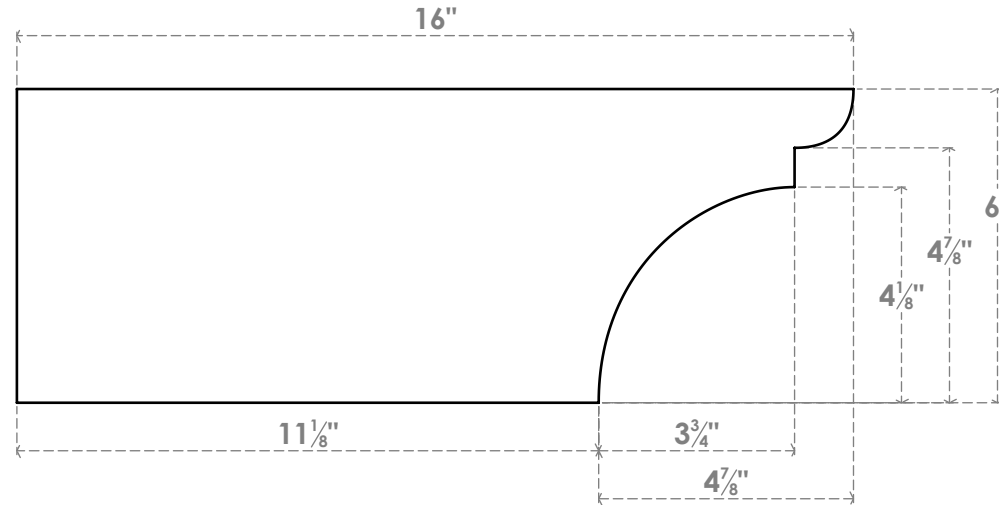
SIDE PROFILE
